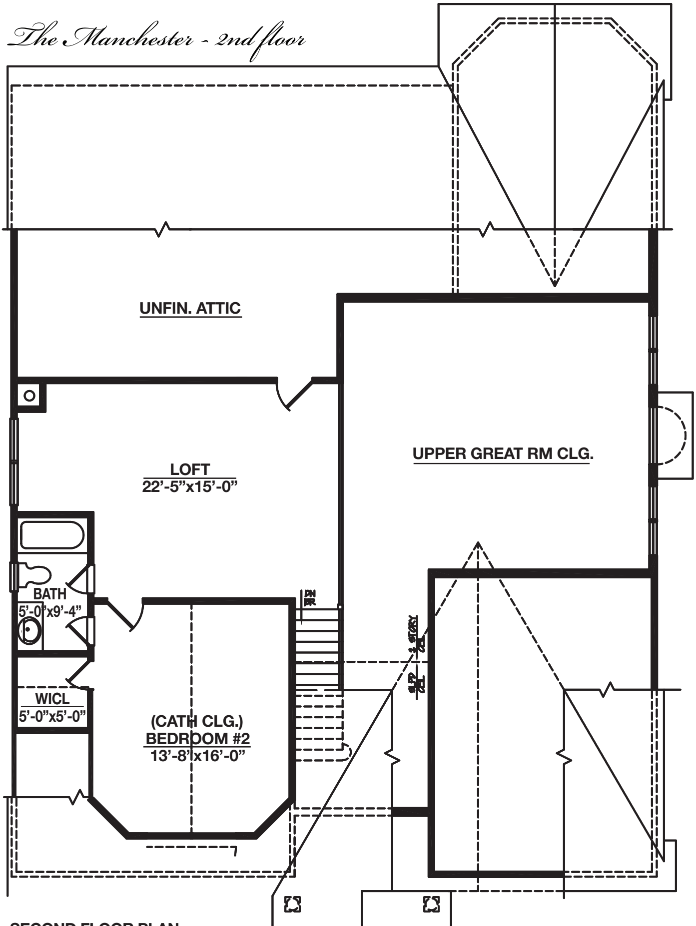
SECOND FLOOR PLAN LIVING AREA: 681 SQ. FT. All dimensions are approximate
